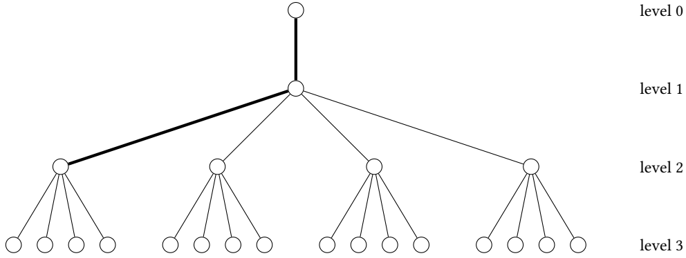
Fig. 2. A tree example which shows that the lower bound of the integrality gap of UFP-ALLRANKTREE is \Omega(\sqrt{\log(n)}) . The thick solid line shown in the figure denotes a request from a vertex to the root.
