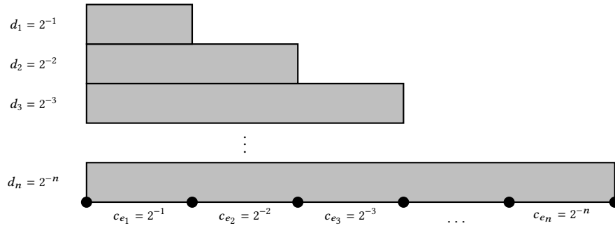
Fig. 1. A canonical example which shows that the lower bound of the integrality gap of UFP-TREE without NBA is \Omega(n) .
